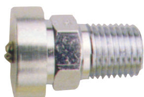
Primary Relief Valve C-21, 31, 41 1/8" 22 PSI Part # PBC-PRV1
