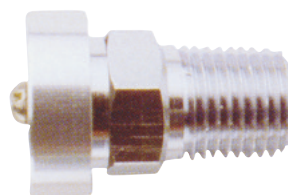
Secondary Relief Valve C-21, 31, 41 1/4" 30 PSI Part # PBC-PRV3
