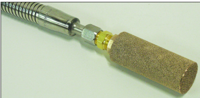
Armored Hose CGA-295 with 1/2" Diffuser with Adapter
