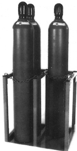
Pt # CBR-M4 Height: 30” Depth: 20” Width: 28.5” Weight: 55 lbs. Cylinder Capacity: 4
