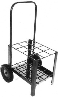
Pt # CBR-DE12T Height: 42" Depth: 20" Width: 22" Weight: 39 lbs. Wheel Dia: 10 x 1.75 Semi-Pneumatic Cylinder Capacity: 12
