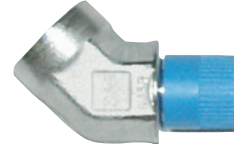
1/4" Female NPT x 1/4" Male NPT Part # FIT-SS45SEF14M14
