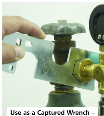
Use as a Captured Wrench - Stays with Regulator
