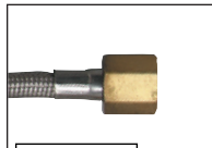
1/4" NPT
